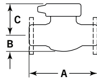
1" & 2" Globe Body
